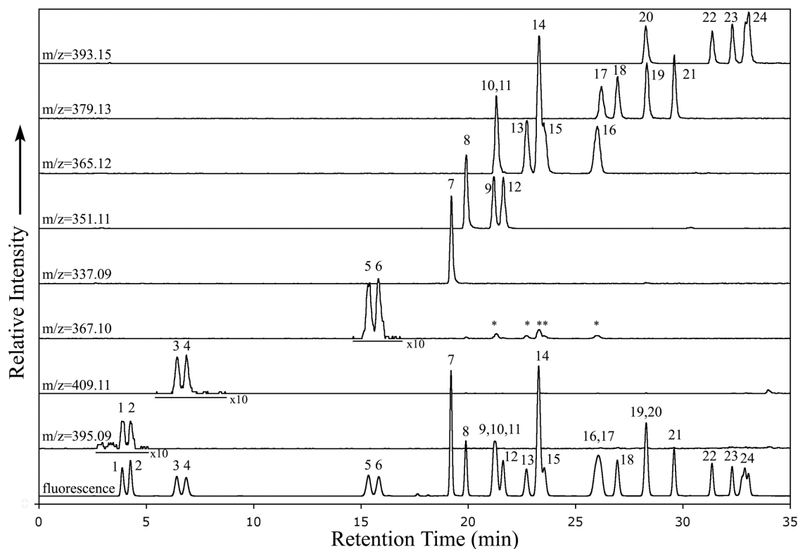
Fig. 1. The 0–35 min region of the HPLC-FD and LC-ToF-MS chromatograms obtained from a single injection of a mixture of OPA/NAC labeled (15 min derivatization) amino acid standards (~10 pmol of each compound). Amino acid peak identifications are given in Table 1. The UV fluorescence trace is shown at the bottom and the exact mass traces were obtained simultaneously in positive electrospray mode for the individual amino acid standards. A detection limit for these amino acids using both UV fluorescence and ToF-MS was determined to be about 10^{-15} – 10^{-16} mol (S/N ~30). The conditions for amino acid separations for the mobile phase at 30 °C were as follows: flow rate, 1 ml/min; solvent A (water); solvent B (methanol); solvent C (50 mM ammonium formate, 8% methanol, pH 8.0); gradient 0–5 min, 100% C; 5–15 min, 0–83% A and 0–12% B; 15–22 min, 83–75% A and 12–20% B; 22–35 min, 75–35% A and 20–60% B. Peaks 1–6 were magnified tenfold due to suppression of the ionization efficiency under highly aqueous conditions during this stage of the HPLC gradient. The asterisks in the 367.10 m/z mass trace correspond to OPA/NAC labeled aminobutyric acids (peaks 10, 11, 13–16) with two naturally occurring ^{13}\text{C} atoms. A similar figure was obtained from negative electrospray mode (data not shown).
